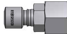
TFS-R Termination Female Straight - BSP page 168
